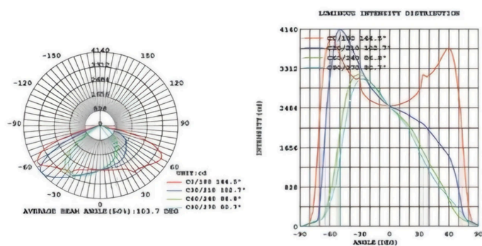
PDZ-60W5700K2MODE
