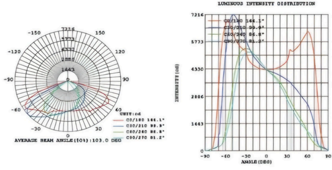
PDZ-100W5700K3MODE
