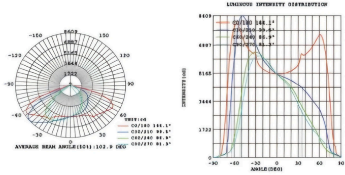
PDZ-120W5700K3MODE
