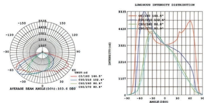
PDZ-80W5700K2MODE
